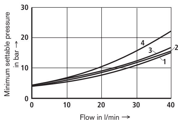
p_{E \min} - q_V - characteristic curves
