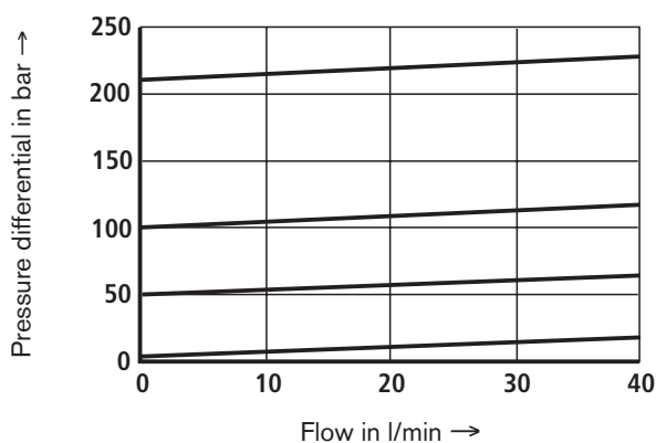
p_E - q_V - characteristic curves
